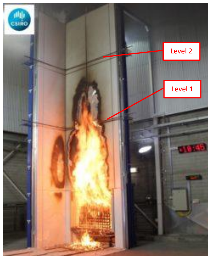
Figure 2. AS5113 thermocouple locations (left), Example of CSIRO AS5113/BS8414 test rig (right)
