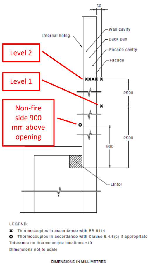
Figure 2. AS5113 thermocouple locations (left), Example of CSIRO AS5113/BS8414 test rig (right)
