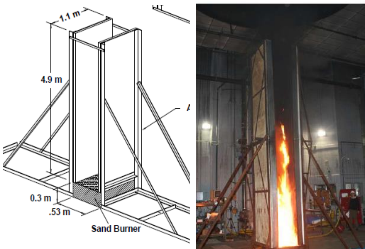
Figure 77. FM Global Parallel Panel Test [153]
