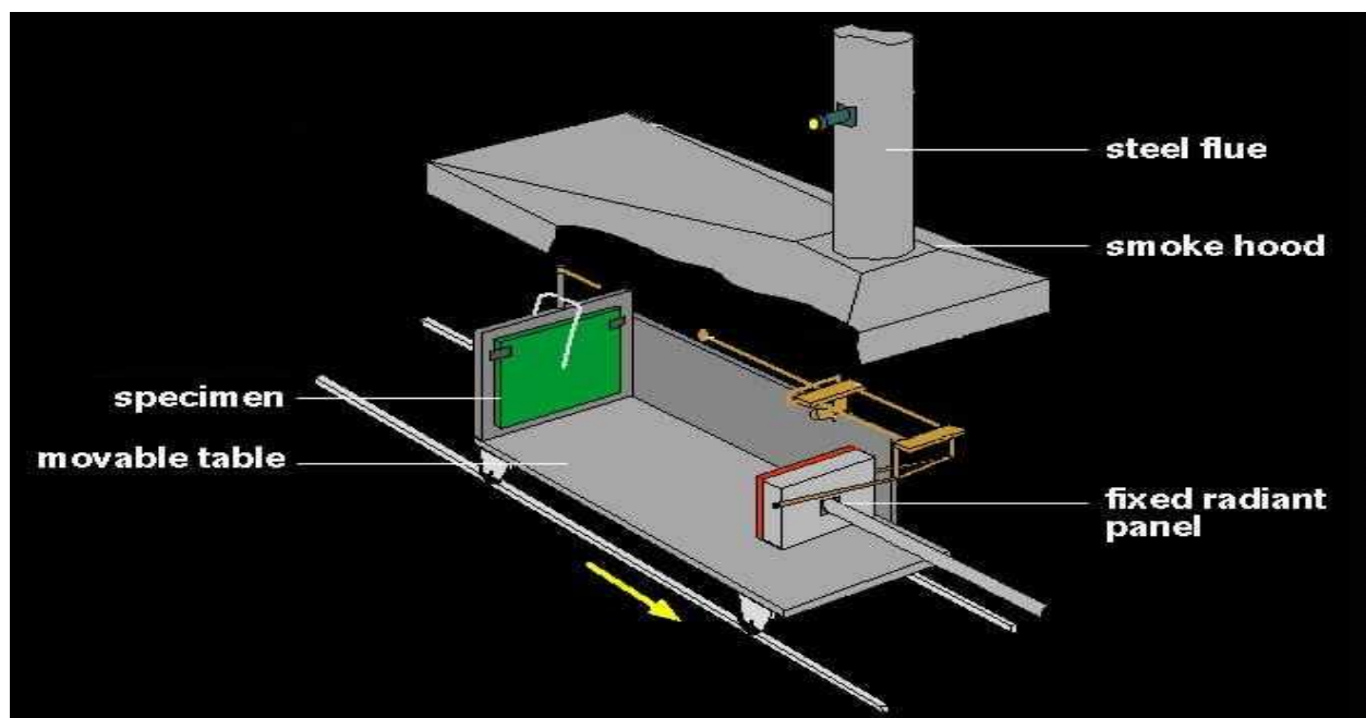
Figure 67 AS 1530.3 test.
