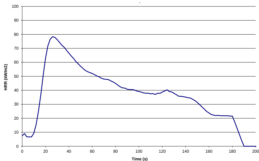
Figure 25. HRRPUA vs time for 50 mm Compolcrete tested to AS 3837 cone calorimeter at 50 \text{ kW/m}^2
