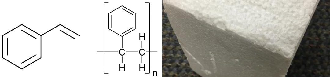
Figure 22. Molecular diagram for styrene monomer (left) and polystyrene (centre). EPS photo (right) by CSIRO.
