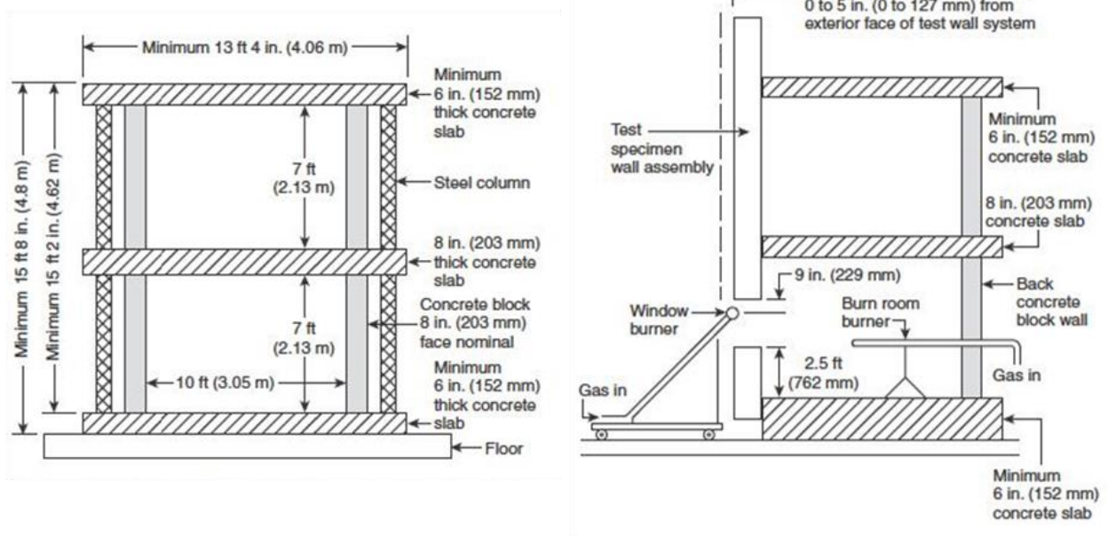
Figure 82. NFPA 285 test apparatus front view without test wall (left) and side view (right) (from NFPA 285-2012) [161]
