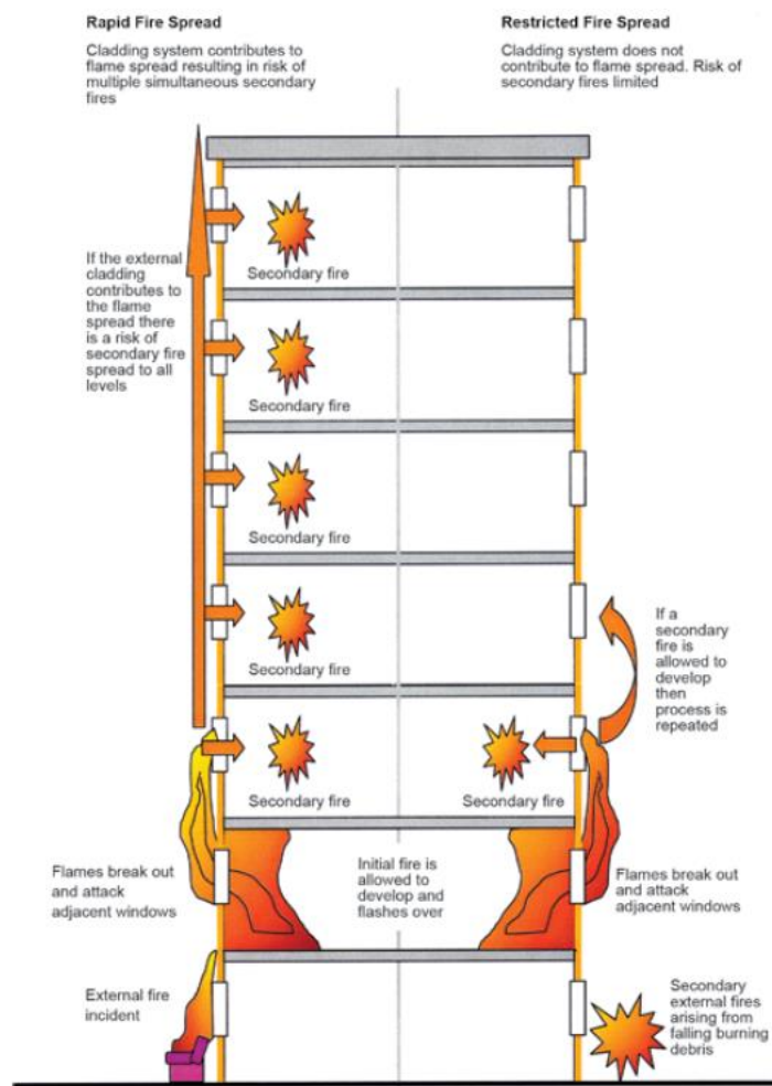
Figure 28. Mechanisms if combustible external wall fire spread [70]
