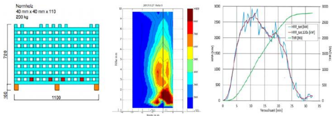
Figure 86. 200 kg crib dimensions, temperature profile and HRR against non-combustible façade [167]
